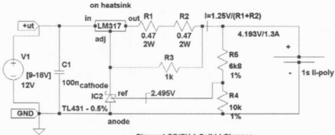
Simplest CC/CV 1 Cell Li Charger
