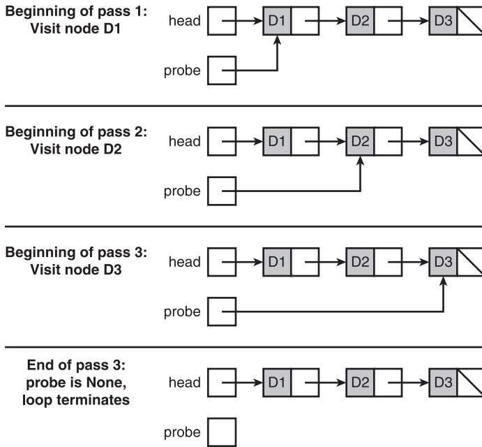
Figure 4.10 Traversing a linked structure. © 2014 Cengage Learning®
