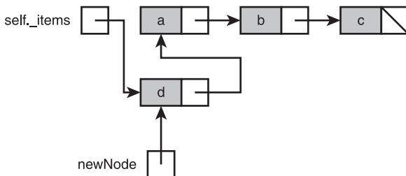
Figure 7.7 Pushing an item onto a linked stack. © 2014 Cengage Learning®
