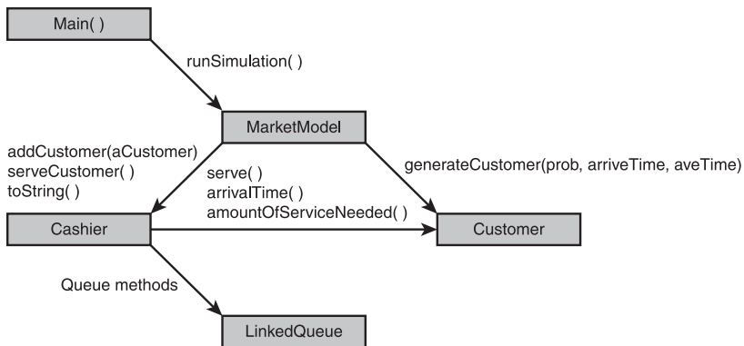
Figure 8.9 A collaboration diagram for the supermarket checkout simulator. © 2014 Cengage Learning®
