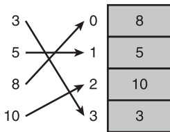
Figure 11.4 Placement of the keys 3, 5, 8, and 10 using the hashing function \text{key} \% 4 . © 2014 Cengage Learning®
