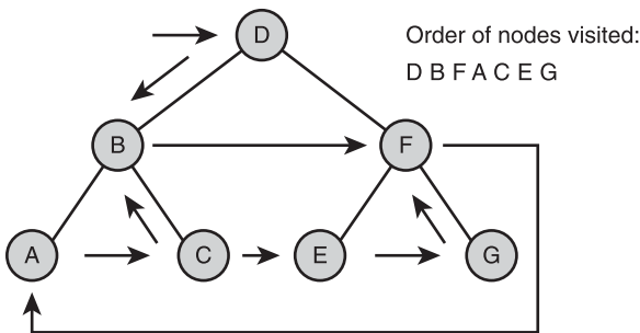
Figure 10.15 A level order traversal. © 2014 Cengage Learning®
