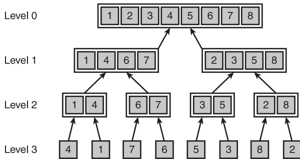
Figure 3.14 Merging the sublists generated during a merge sort.
