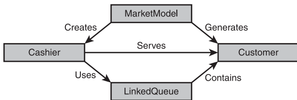
Figure 8.8 A class diagram of the supermarket checkout simulator. © 2014 Cengage Learning®
