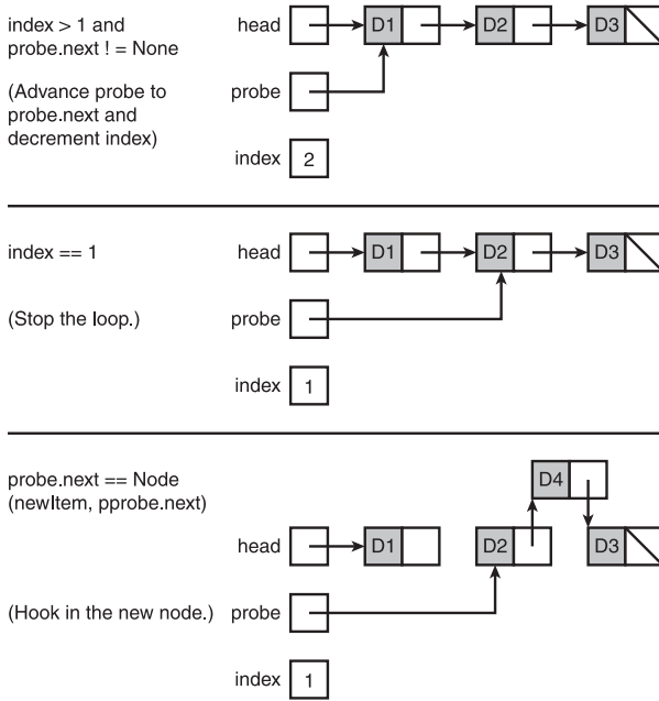
Figure 4.15 Inserting an item between two items in a linked structure. © 2014 Cengage Learning®
