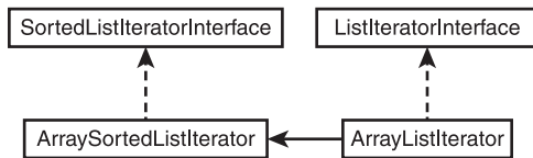
Figure 9.9 An implementation strategy for array-based list iterators.
