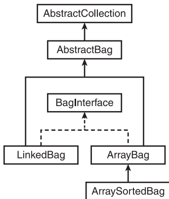
Figure 6.3 Adding an abstract collection class to the collection framework.
