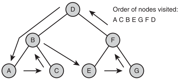
Figure 10.14 A postorder traversal. © 2014 Cengage Learning®
