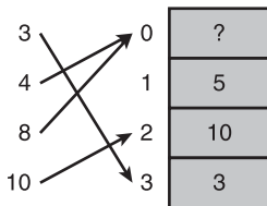
Figure 11.5 Placement of the keys 3, 4, 8, and 10 using the hashing function \text{key} \% 4 . © 2014 Cengage Learning®
